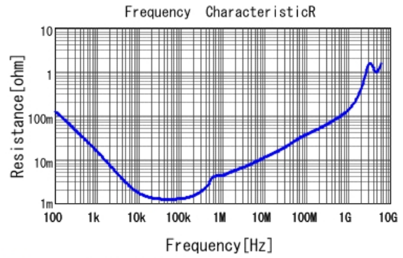
■ GRM31CC80E227ME11 R DCOV, 25degC
