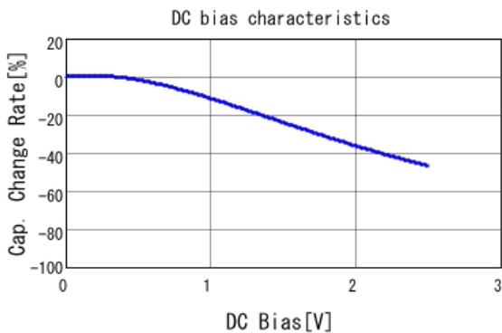
■ GRM31CC80E227ME11 C-DC bias capchange, 25.0degC, AC0.
