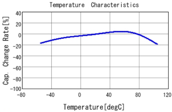
■ GRM31CC80E227ME11 C-Temp. capchange, DC0.0V, AC0.05Vr
