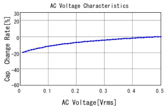
■ GRM31CC80E227ME11 C-AC Voltage capchange, DCOV, 25.0d
