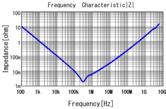
■ GRM31CC80E227ME11 |Z| DCOV, 25degC
