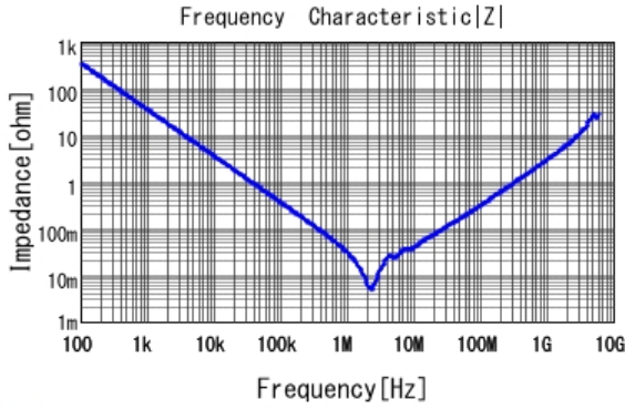
■ GRM31CC72A475ME11 |Z| DCOV, 25degC
