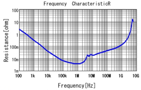
■ GRM31CC72A475ME11 R DCOV, 25degC
