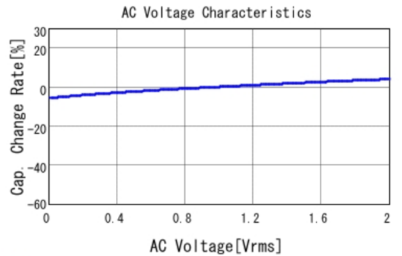
■ GRM31CC72A475ME11 C-AC Voltage capchange, DCOV, 25.0d
