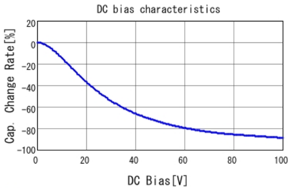
■ GRM31CC72A475ME11 C-DC bias capchange, 25.0degC, AC1V
