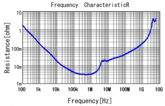
■ GRM31CB31H475KA12 R DCOV, 20degC
