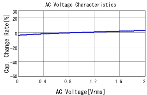
■ GRM31CB31H475KA12 C-AC Voltage capchange, DCOV, 20.0d
