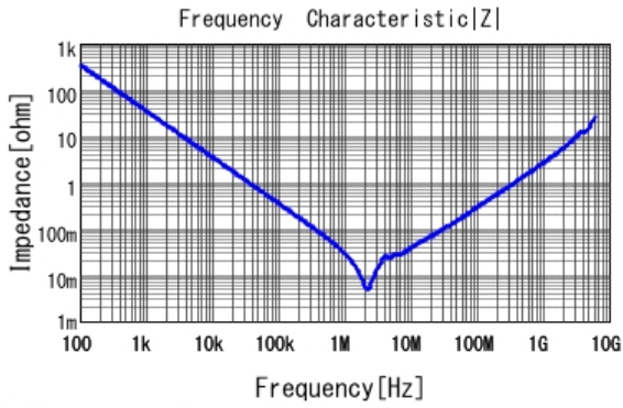
■ GRM31CB31H475KA12 |Z| DCOV, 20degC
