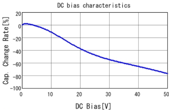
■ GRM31CB31H475KA12 C-DC bias capchange, 20.0degC, AC1.
