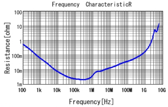
■ GRM31CB30J476ME18 R DCOV, 20degC
