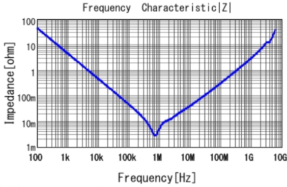
■ GRM31CB30J476ME18 |Z| DCOV, 20degC
