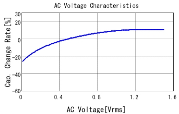
■ GRM31CB30J476ME18 C-AC Voltage capchange, DCOV, 20.0d
