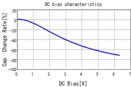
■ GRM31CB30J476ME18 C-DC bias capchange, 20.0degC, AC0.
