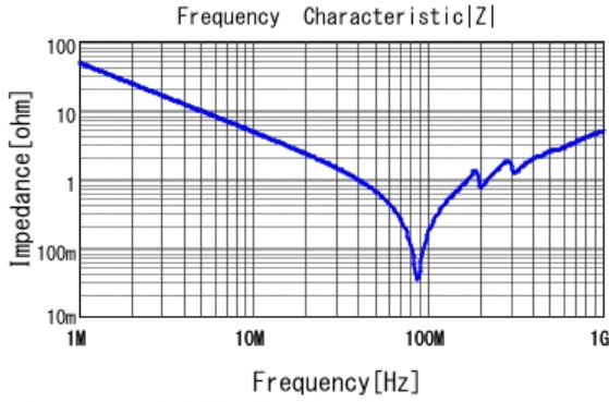
■ GRM31C5C2J332JWA3 |Z| DCOV, 25degC
