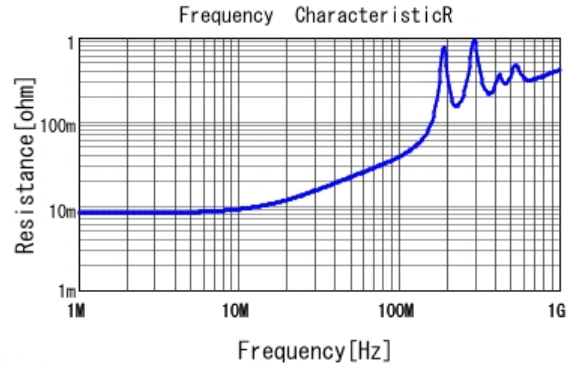
■ GRM31C5C2J332JWA3 R DCOV, 25degC
