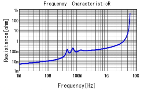
■ GRM31C5C2A683JA01 R DCOV, 25degC
