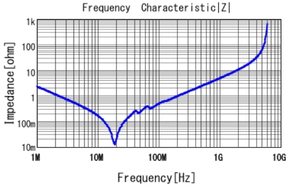
■ GRM31C5C2A683JA01 |Z| DCOV, 25degC
