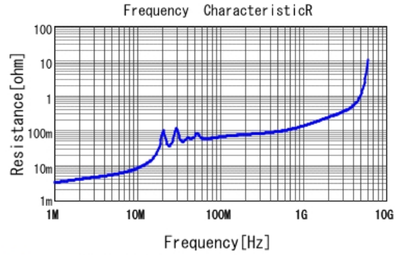
■ GRM31C5C1E224JE02 R DCOV, 25degC
