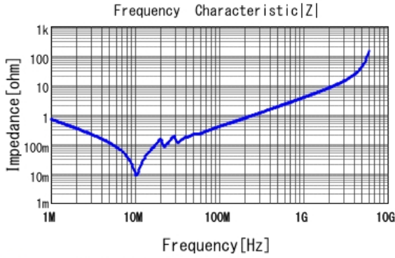
■ GRM31C5C1E224JE02 |Z| DCOV, 25degC
