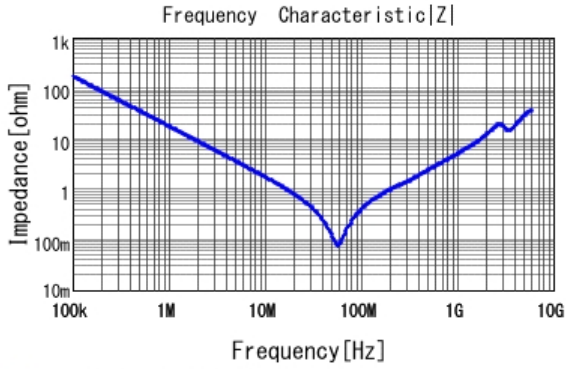
■ GRM31BR72J103KW01 |Z| DCOV, 25degC
