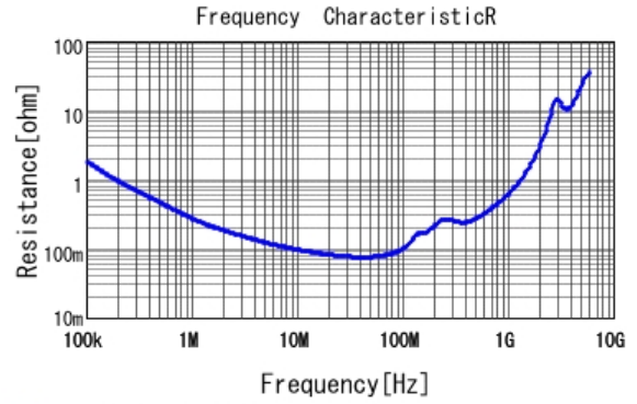
■ GRM31BR72J103KW01 R DCOV, 25degC
