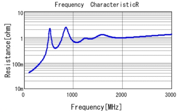
■ GRM31B7U3A561JW31 R DCOV, 25degC
