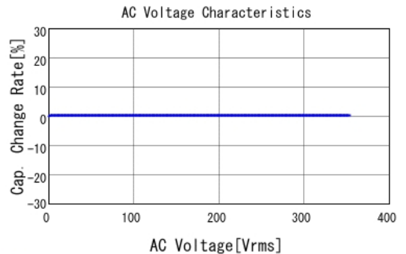
■ GRM31B7U3A561JW31 C-AC Voltage capchange, DCOV, 25.0d
