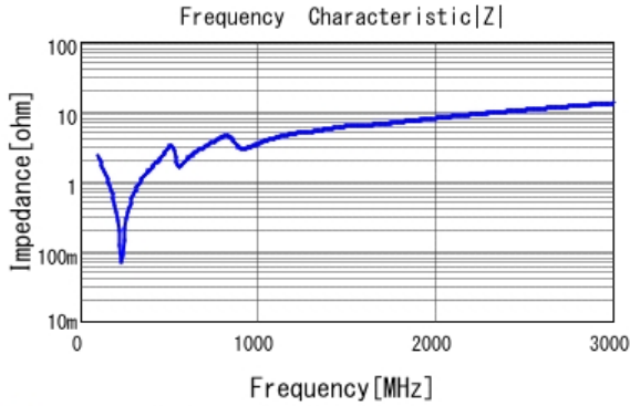
■ GRM31B7U3A561JW31 |Z| DCOV, 25degC
