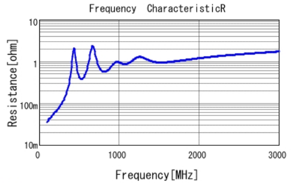
■ GRM31B5C3A681JWA1 R DCOV, 25degC
