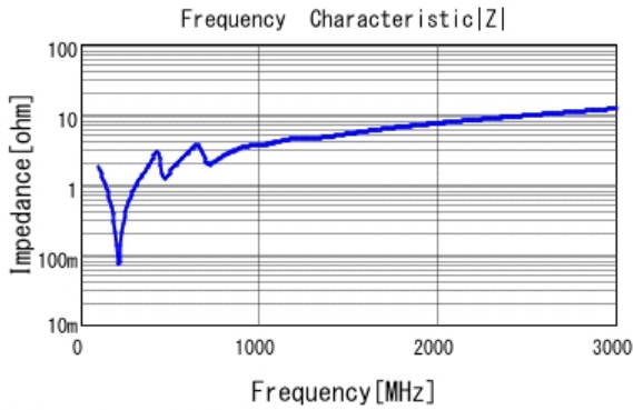
■ GRM31B5C3A681JWA1 |Z| DCOV, 25degC
