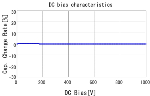
■ GRM31B5C3A681JWA1 C-DC bias capchange, 25.0degC, AC1V
