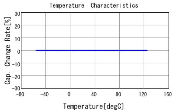
■ GRM31B5C3A681JWA1 C-Temp. capchange, DCOV, AC1Vrms
