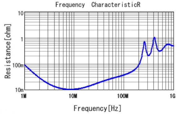
■ GRM31B5C2J222JWA1 R DCOV, 25degC
