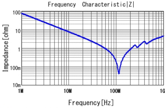
■ GRM31B5C2J222JWA1 |Z| DCOV, 25degC
