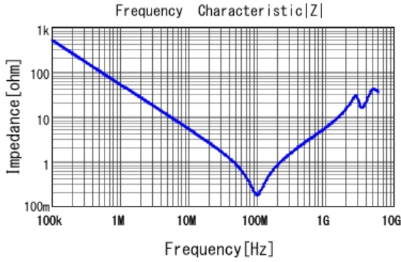
■ GRM31AR72J332KW01 |Z| DCOV, 25degC
