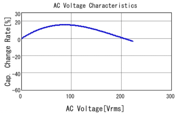
■ GRM31AR72J332KW01 C-AC Voltage capchange, DCOV, 25.0d
