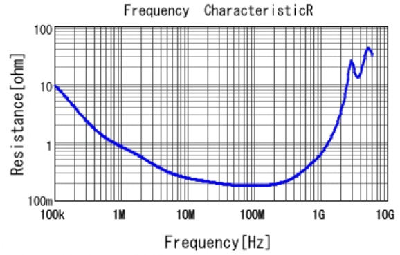
■ GRM31AR72J332KW01 R DCOV, 25degC
