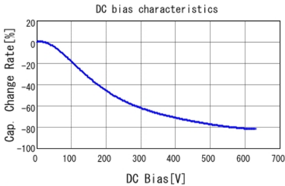
■ GRM31AR72J332KW01 C-DC bias capchange, 25.0degC, AC1V
