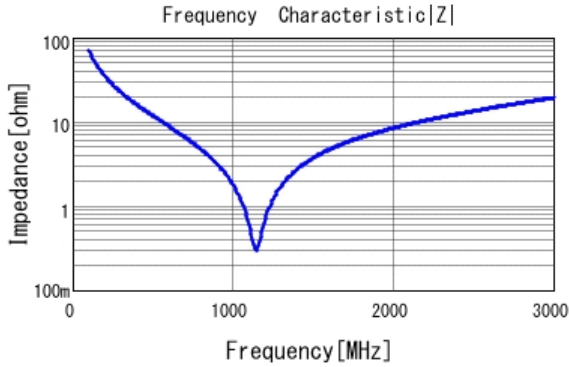
■ GRM31A7U3D220JW31 |Z| DC0V, 25degC
