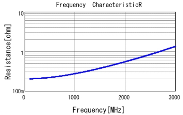
■ GRM31A7U3D220JW31 R DC0V, 25degC
