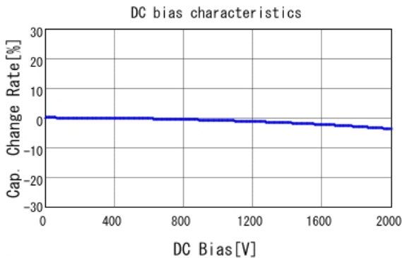
■ GRM31A7U3D220JW31 C-DC bias capchange, 25.0degC, AC1V
