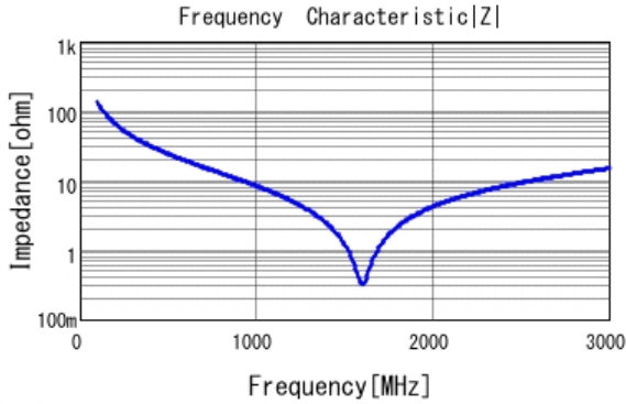
■ GRM31A7U3D120JW31 |Z| DCOV, 25degC
