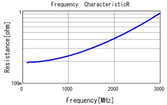
■ GRM31A7U3D120JW31 R DCOV, 25degC
