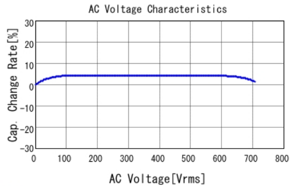
■ GRM31A7U3D120JW31 C-AC Voltage capchange, DCOV, 25.0d
