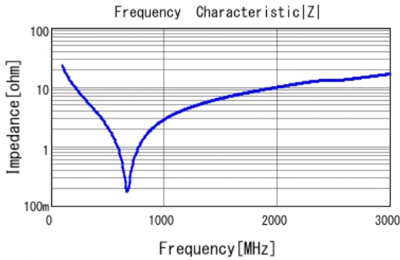
■ GRM31A5C2J680JW01 |Z| DCOV, 25degC
