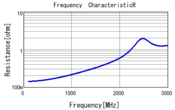
■ GRM31A5C2J680JW01 R DCOV, 25degC
