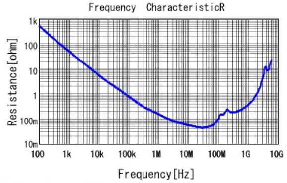
■ GRM319R72A153KA01 R DCOV, 25degC
