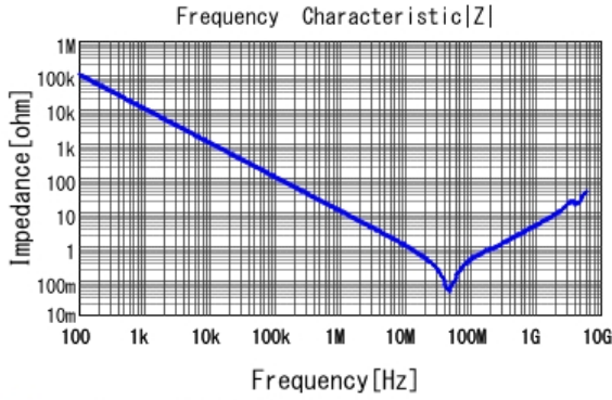
■ GRM319R72A153KA01 |Z| DCOV, 25degC
