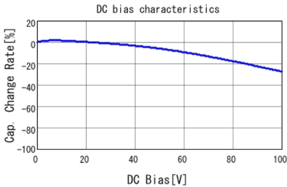
■ GRM319R72A153KA01 C-DC bias capchange, 25.0degC, AC1.
