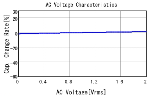
■ GRM319R72A153KA01 C-AC Voltage capchange, DCOV, 25.0d
