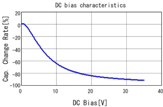
■ GRM319R6YA106MA12 C-DC bias capchange, 25.0degC, AC1.
