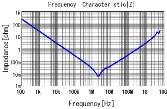
■ GRM319R6YA106MA12 |Z| DCOV, 25degC
