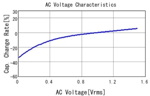
■ GRM319R6YA106MA12 C-AC Voltage capchange, DCOV, 25.0d
