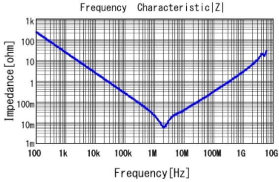
■ GRM319R61E106MA12 |Z| DCOV, 25degC
