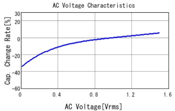
■ GRM319R61E106MA12 C-AC Voltage capchange, DCOV, 25.0d
