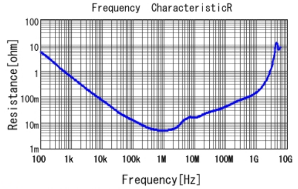
■ GRM319R61E106MA12 R DCOV, 25degC
