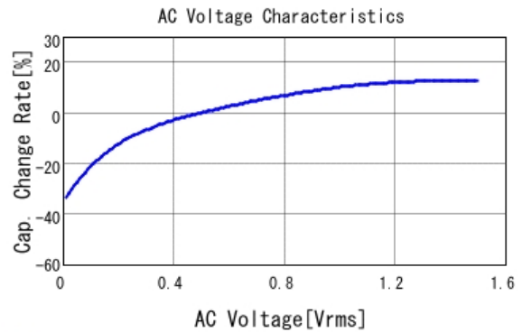
■ GRM319R61C226ME15 C-AC Voltage capchange, DCOV, 25.0d
