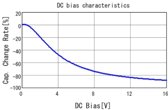
■ GRM319R61C226ME15 C-DC bias capchange, 25.0degC, AC0.
