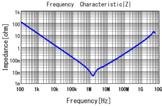
■ GRM319R61C226ME15 |Z| DCOV, 25degC
