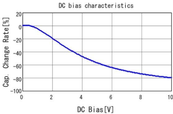
■ GRM319R61A226ME15 C-DC bias capchange, 25.0degC, AC0.
