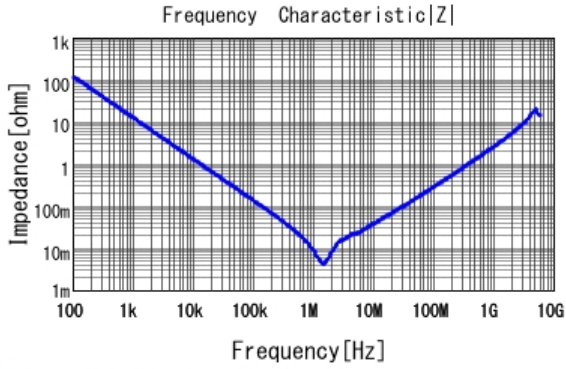
■ GRM319R61A226ME15 |Z| DCOV, 25degC
