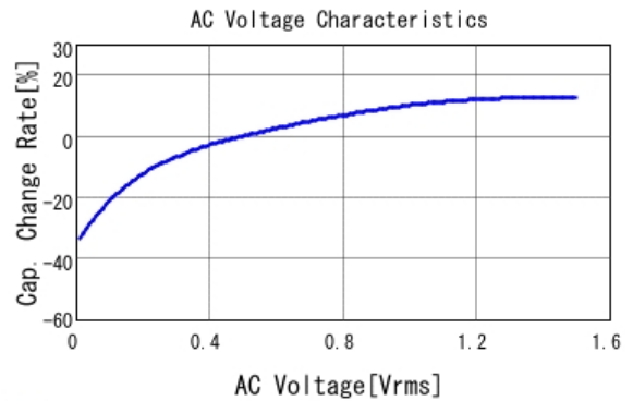
■ GRM319R61A226ME15 C-AC Voltage capchange, DCOV, 25.0d
