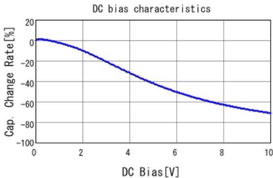
■ GRM319R61A106KE19 C-DC bias capchange, 25.0degC, AC0.
