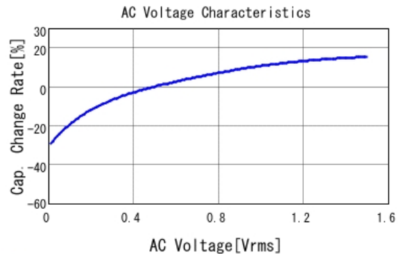
■ GRM319R61A106KE19 C-AC Voltage capchange, DCOV, 25.0d
