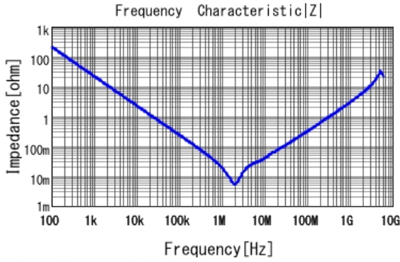
■ GRM319R61A106KE19 |Z| DCOV, 25degC
