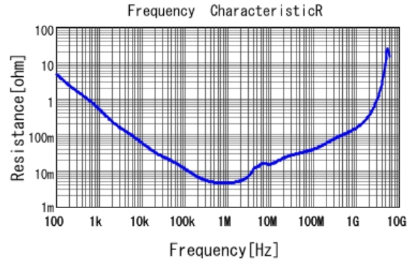
■ GRM319R61A106KE19 R DCOV, 25degC
