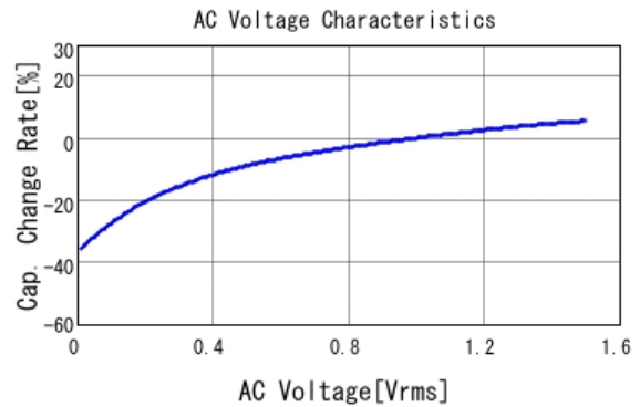
■ GRM319C81C106MA12 C-AC Voltage capchange, DCOV, 25.0d
