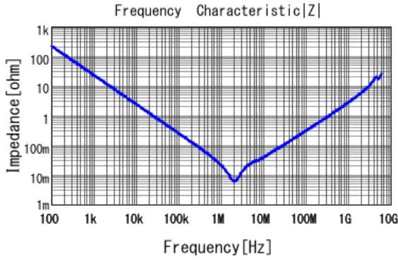
■ GRM319C81C106MA12 |Z| DCOV, 25degC
