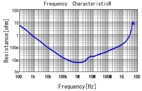
■ GRM319C81C106MA12 R DCOV, 25degC
