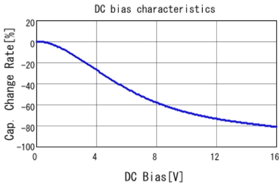
■ GRM319C81C106MA12 C-DC bias capchange, 25.0degC, AC1V
