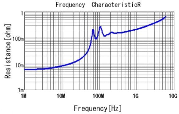
■ GRM3195C2A333JA01 R DCOV, 25degC
