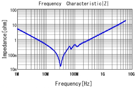
■ GRM3195C2A333JA01 |Z| DCOV, 25degC
