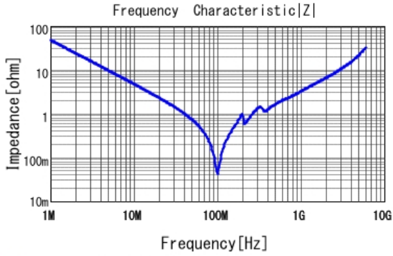
■ GRM3195C2A332JA01 |Z| DCOV, 25degC
