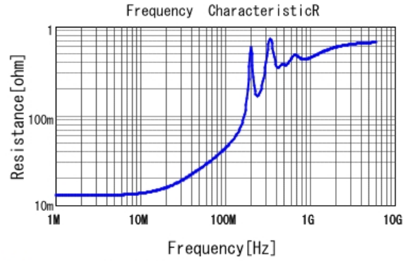
■ GRM3195C2A332JA01 R DCOV, 25degC
