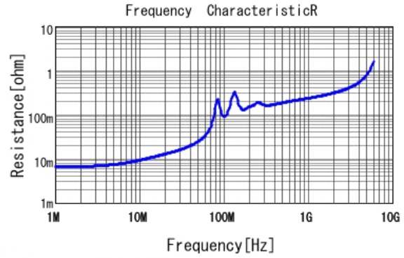
■ GRM3195C2A223JA01 R DCOV, 25degC
