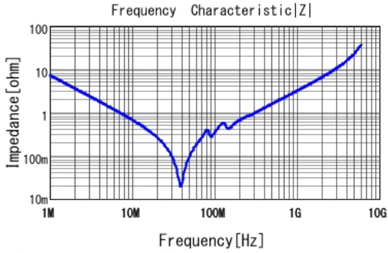
■ GRM3195C2A223JA01 |Z| DCOV, 25degC
