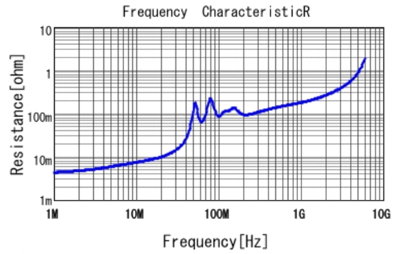
■ GRM3195C1H563JA05 R DCOV, 25degC
