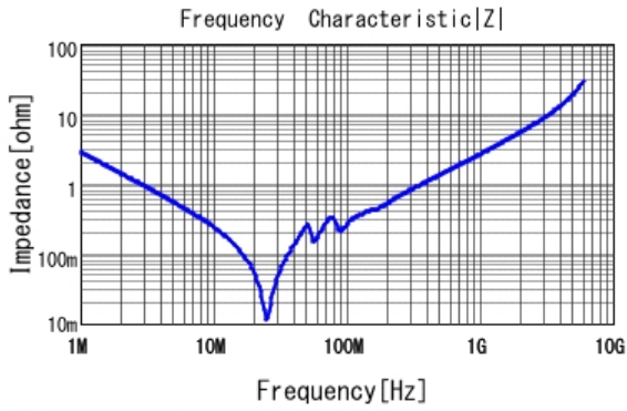
■ GRM3195C1H563JA05 |Z| DCOV, 25degC
