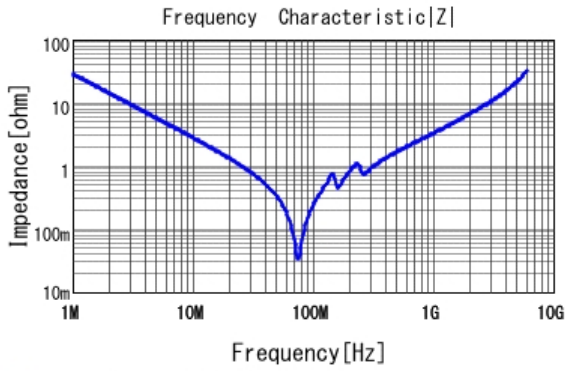
■ GRM3195C1H562JA01 |Z| DCOV, 25degC
