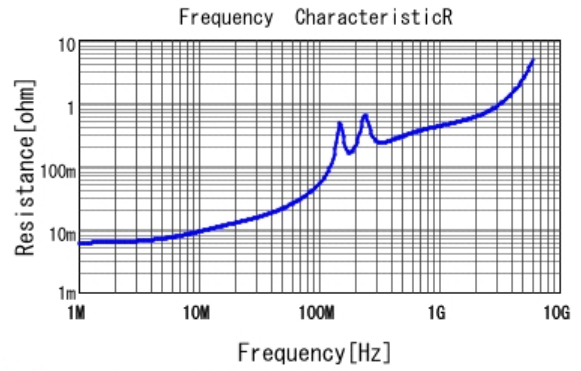
■ GRM3195C1H562JA01 R DCOV, 25degC
