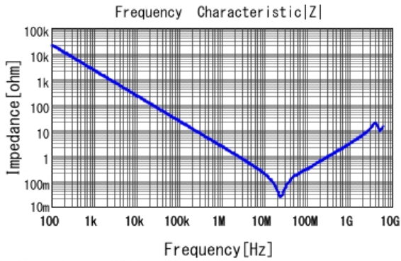
■ GRM21BR72A683KAC4 |Z| DCOV, 25degC
