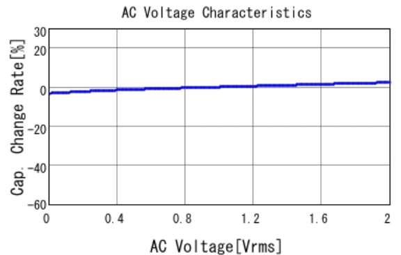
■ GRM21BR72A683KAC4 C-AC Voltage capchange, DCOV, 25.0d
