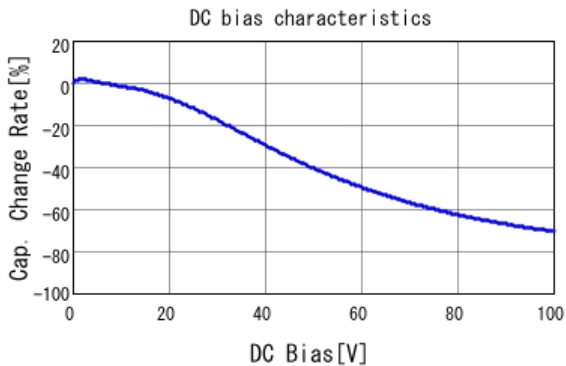
■ GRM21BR72A683KAC4 C-DC bias capchange, 25.0degC, AC1.
