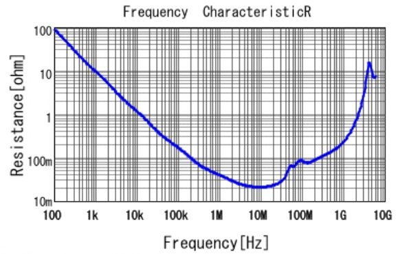
■ GRM21BR72A683KAC4 R DCOV, 25degC
