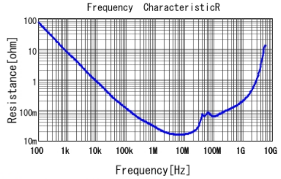
■ GRM21BR72A104KAC4 R DCOV, 25degC
