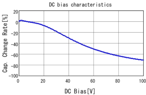
■ GRM21BR72A104KAC4 C-DC bias capchange, 25.0degC, AC1.
