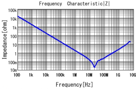
■ GRM21BR72A104KAC4 |Z| DCOV, 25degC
