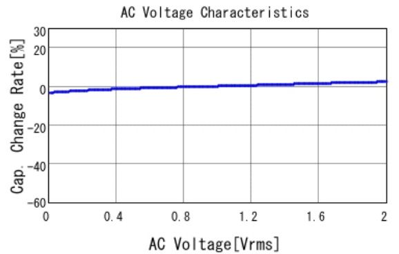
■ GRM21BR72A104KAC4 C-AC Voltage capchange, DCOV, 25.0d
