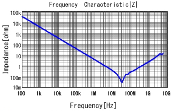
■ GRM21BR71H473KA01 |Z| DCOV, 25degC
