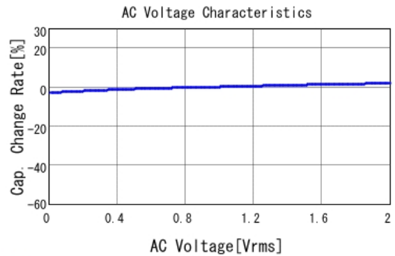
■ GRM21BR71H473KA01 C-AC Voltage capchange, DCOV, 25.0d
