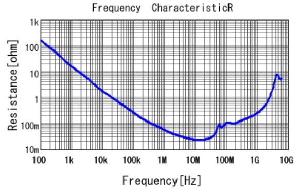
■ GRM21BR71H473KA01 R DCOV, 25degC
