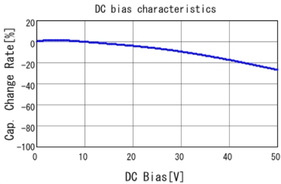
■ GRM21BR71H473KA01 C-DC bias capchange, 25.0degC, AC1.
