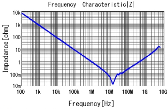
■ GRM21BR71H224MA01 |Z| DCOV, 25degC
