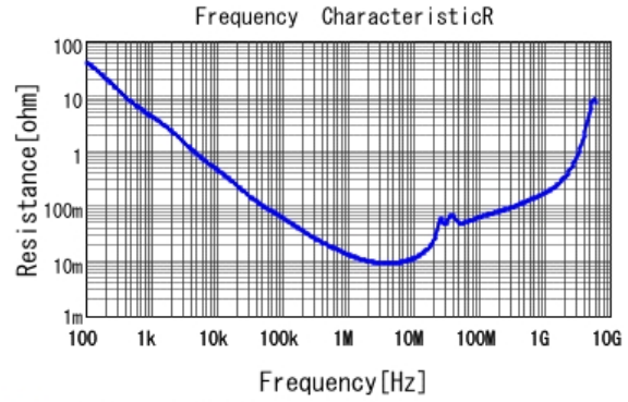
■ GRM21BR71H224MA01 R DCOV, 25degC
