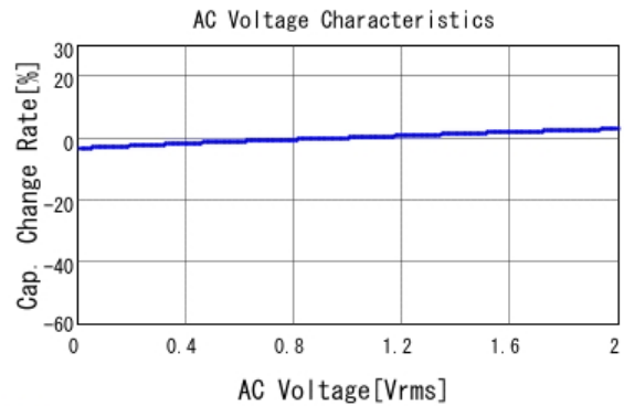
■ GRM21BR71H224MA01 C-AC Voltage capchange, DCOV, 25.0d
