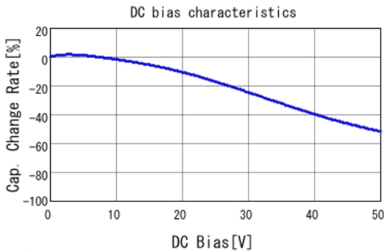
■ GRM21BR71H224MA01 C-DC bias capchange, 25.0degC, AC1.
