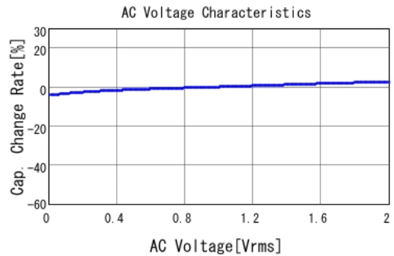
■ GRM21BR71E224KA01 C-AC Voltage capchange, DCOV, 25.0d
