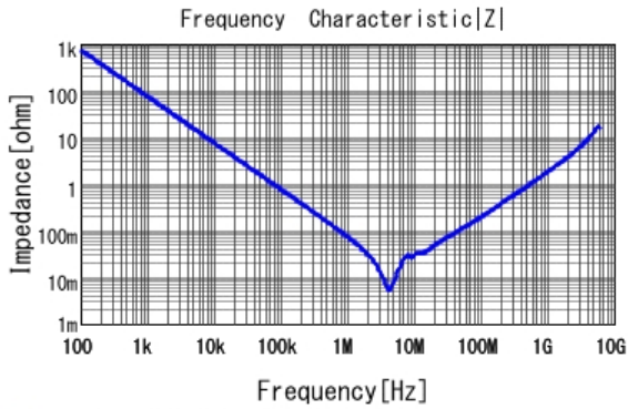
■ GRM21BR71A225MA01 |Z| DCOV, 25degC
