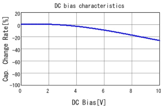
■ GRM21BR71A225MA01 C-DC bias capchange, 25.0degC, AC1.
