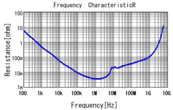
■ GRM21BR71A225MA01 R DCOV, 25degC
