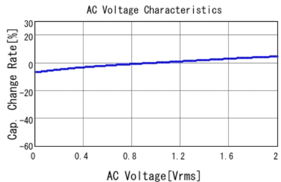
■ GRM21BR71A225MA01 C-AC Voltage capchange, DCOV, 25.0d
