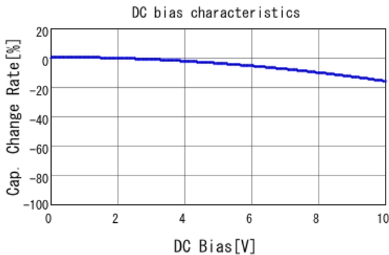
■ GRM21BR71A105KA01 C-DC bias capchange, 25.0degC, AC1.
