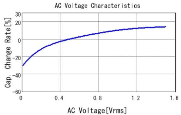
■ GRM21BR61D106ME15 C-AC Voltage capchange, DCOV, 25.0d
