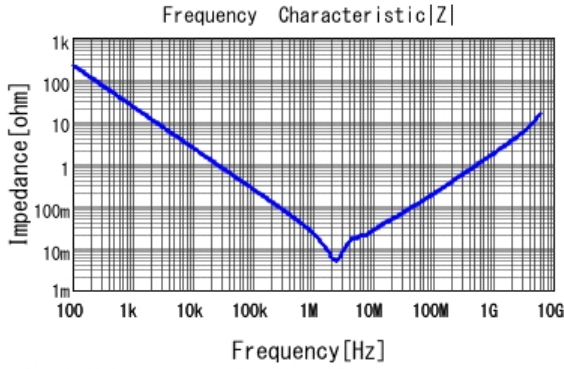
■ GRM21BR61D106ME15 |Z| DCOV, 25degC
