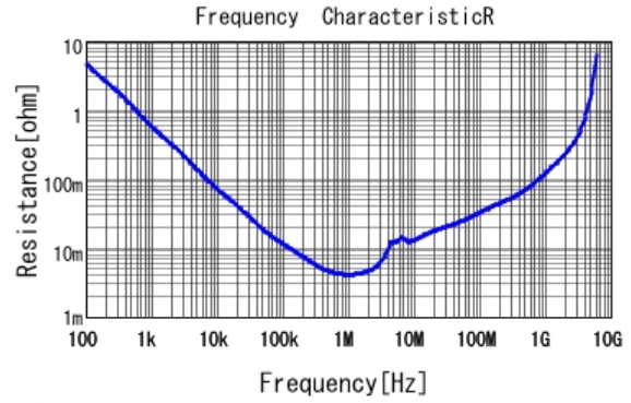
■ GRM21BR61D106ME15 R DCOV, 25degC
