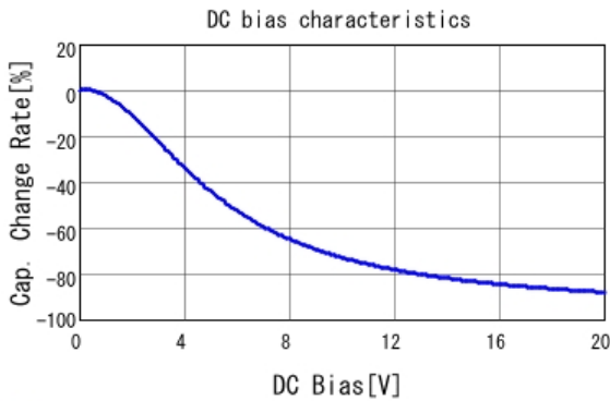
■ GRM21BR61D106ME15 C-DC bias capchange, 25.0degC, AC0.
