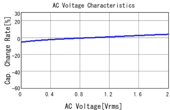
■ GRM21BR61A105KA01 C-AC Voltage capchange, DCOV, 25.0d
