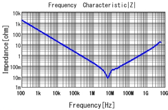
■ GRM21BR61A105KA01 |Z| DCOV, 25degC
