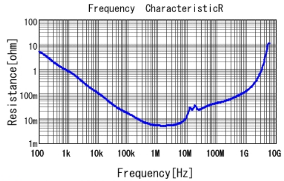
■ GRM21BR61A105KA01 R DCOV, 25degC
