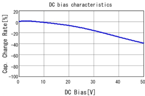
■ GRM21BR11H104KA01 C-DC bias capchange, 20.0degC, AC1.
