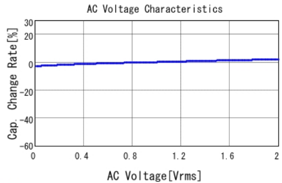
■ GRM21BR11H104KA01 C-AC Voltage capchange, DCOV, 20.0d
