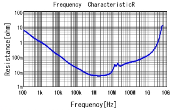
■ GRM21BR11A105KA01 R DCOV, 20degC
