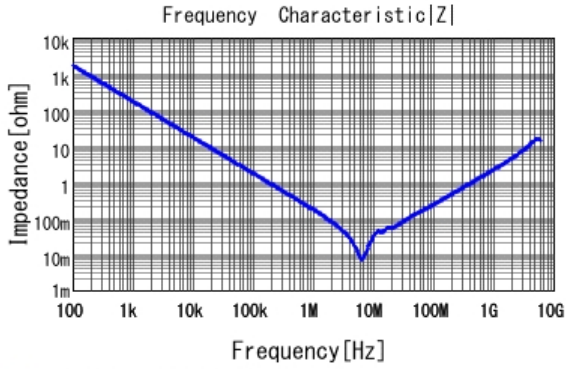
■ GRM21BR11A105KA01 |Z| DCOV, 20degC
