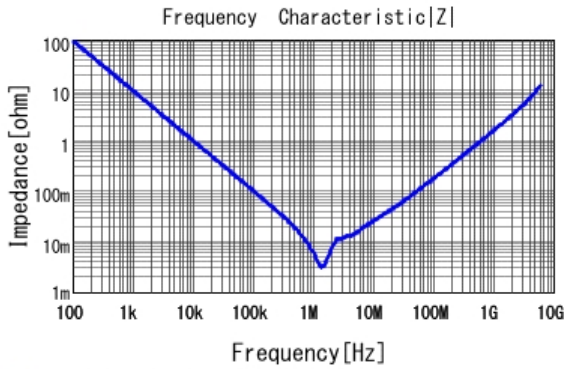
■ GRM21BD70J226ME44 |Z| DCOV, 25degC
