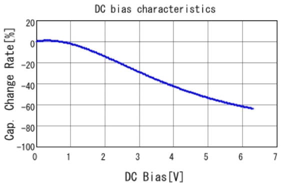
■ GRM21BD70J226ME44 C-DC bias capchange, 25.0degC, AC0.
