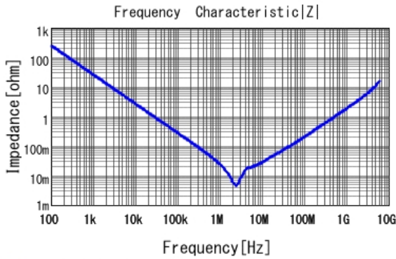
■ GRM21BC81C106MA73 |Z| DCOV, 25degC
