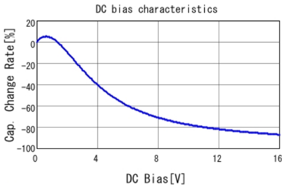
■ GRM21BC81C106MA73 C-DC bias capchange, 25.0degC, AC1.
