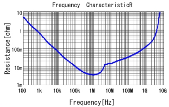
■ GRM21BC81C106MA73 R DCOV, 25degC
