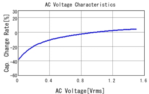
■ GRM21BC81C106MA73 C-AC Voltage capchange, DCOV, 25.0d
