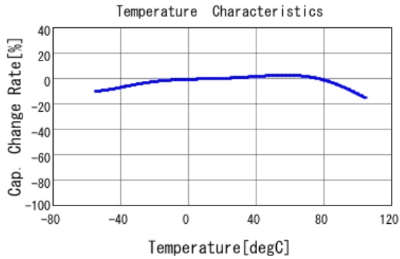
■ GRM21BC80E107ME15 C-Temp. capchange, DC0.0V, AC0.05Vr
