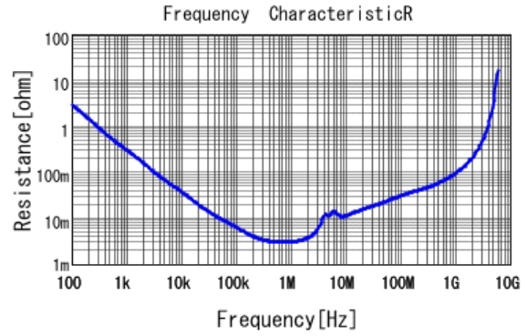
■ GRM21BC71E106ME11 R DCOV, 25degC
