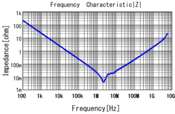
■ GRM21BC71E106ME11 |Z| DCOV, 25degC
