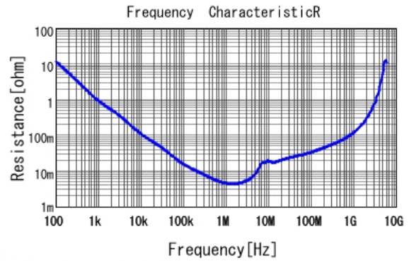
■ GRM21BB31H475KE51 R DCOV, 20degC
