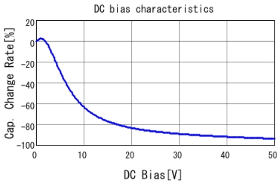
■ GRM21BB31H475KE51 C-DC bias capchange, 20.0degC, AC1.
