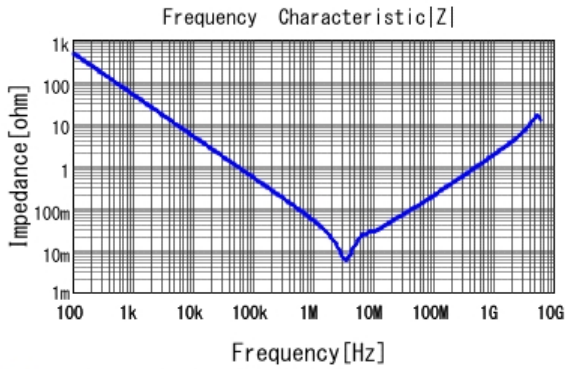
■ GRM21BB31H475KE51 |Z| DCOV, 20degC
