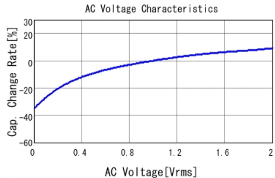
■ GRM21BB31H475KE51 C-AC Voltage capchange, DCOV, 20.0d
