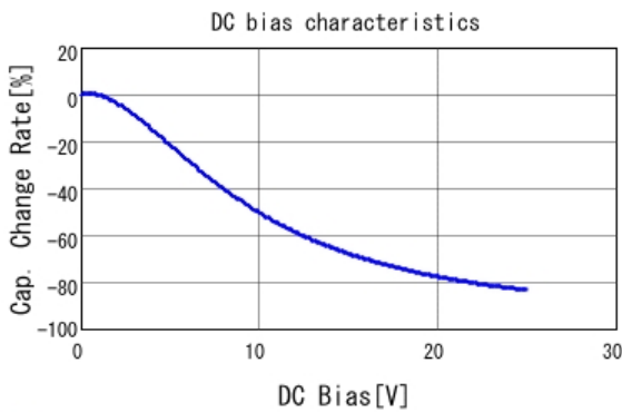
■ GRM21BB31E475KA75 C-DC bias capchange, 20.0degC, AC1.
