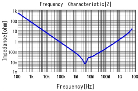
■ GRM21BB31E475KA75 |Z| DCOV, 20degC
