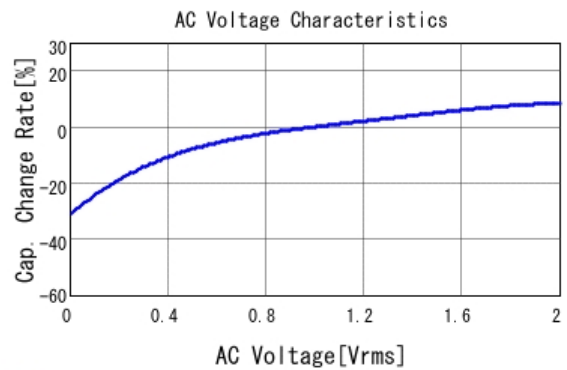
■ GRM21BB31E475KA75 C-AC Voltage capchange, DCOV, 20.0d
