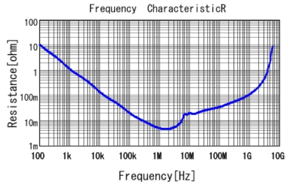
■ GRM21BB31E475KA75 R DCOV, 20degC
