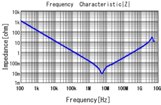
■ GRM21BB31E225KA75 |Z| DCOV, 20degC
