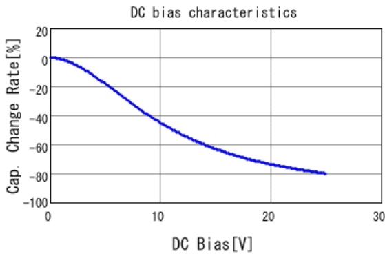
■ GRM21BB31E225KA75 C-DC bias capchange, 20.0degC, AC1.
