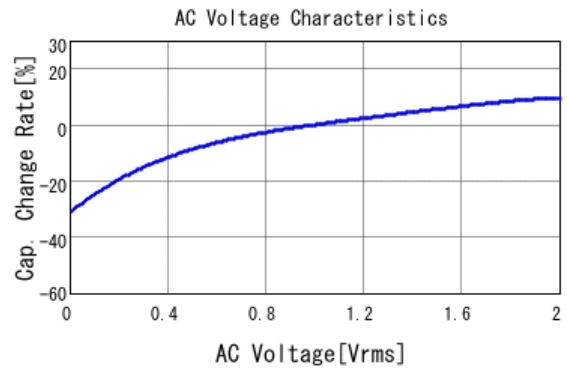
■ GRM21BB31E225KA75 C-AC Voltage capchange, DCOV, 20.0d
