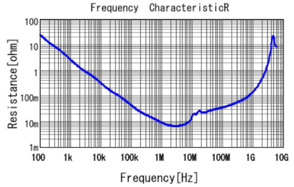
■ GRM21BB31E225KA75 R DCOV, 20degC
