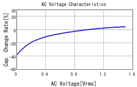
■ GRM21BB31E106KA73 C-AC Voltage capchange, DCOV, 20.0d
