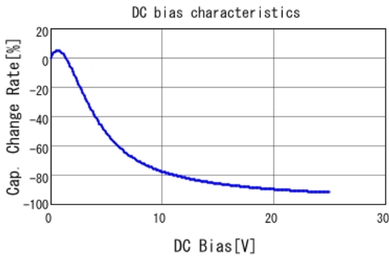
■ GRM21BB31E106KA73 C-DC bias capchange, 20.0degC, AC1.
