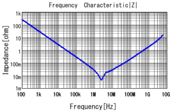
■ GRM21BB31E106KA73 |Z| DCOV, 20degC
