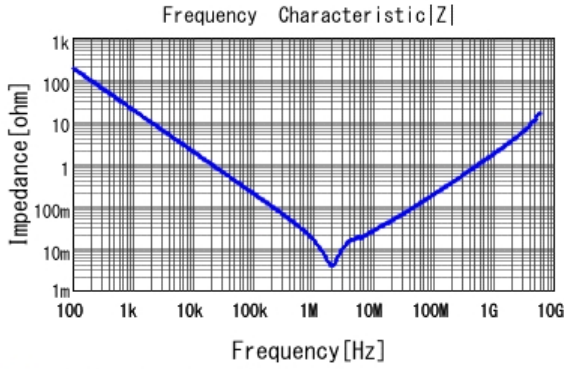
■ GRM21BB31C106KE15 |Z| DCOV, 20degC
