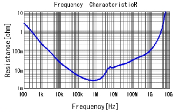
■ GRM21BB31C106KE15 R DCOV, 20degC
