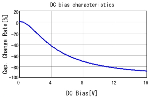
■ GRM21BB31C106KE15 C-DC bias capchange, 20.0degC, AC0.
