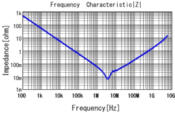
■ GRM21BB31A475KA74 |Z| DCOV, 20degC
