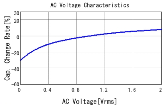
■ GRM21BB31A475KA74 C-AC Voltage capchange, DCOV, 20.0d
