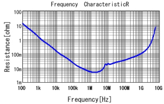
■ GRM21BB31A475KA74 R DCOV, 20degC
