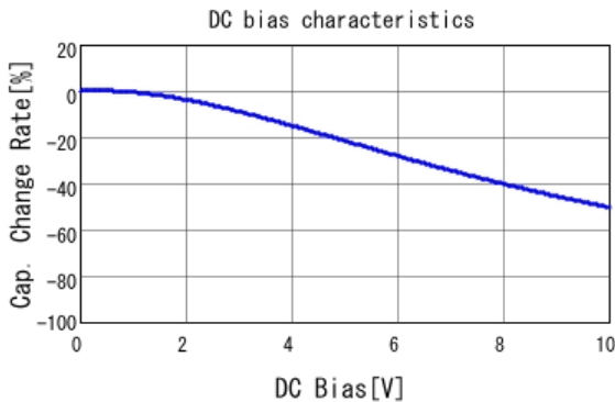
■ GRM21BB31A475KA74 C-DC bias capchange, 20.0degC, AC1.
