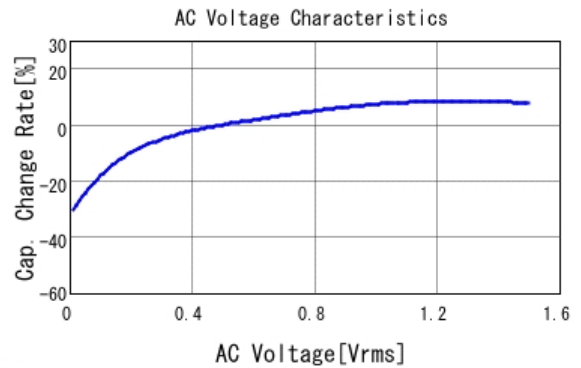
■ GRM21BB31A226ME51 C-AC Voltage capchange, DCOV, 20.0d
