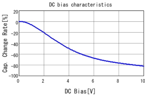
■ GRM21BB31A226ME51 C-DC bias capchange, 20.0degC, AC0.
