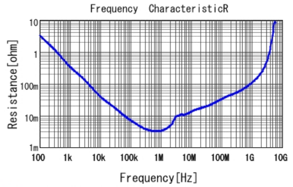
■ GRM21BB31A226ME51 R DCOV, 20degC
