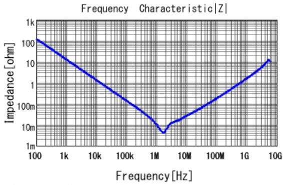
■ GRM21BB31A226ME51 |Z| DCOV, 20degC
