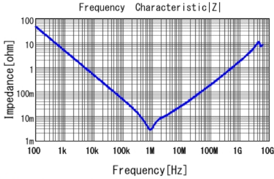
■ GRM21BB30J476ME15 |Z| DCOV, 20degC
