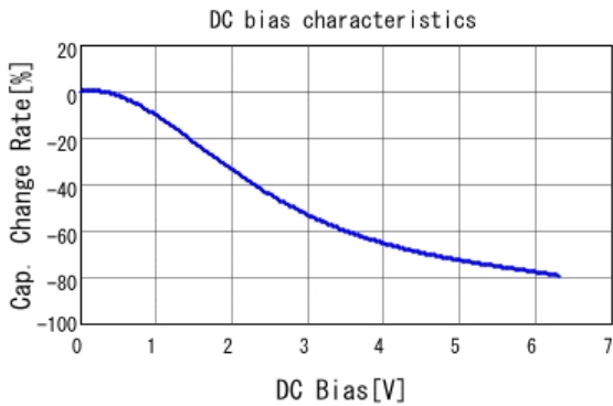
■ GRM21BB30J476ME15 C-DC bias capchange, 20.0degC, AC0.
