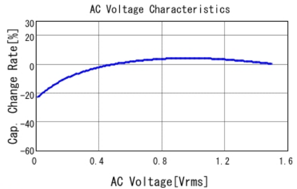
■ GRM21BB30J476ME15 C-AC Voltage capchange, DCOV, 20.0d
