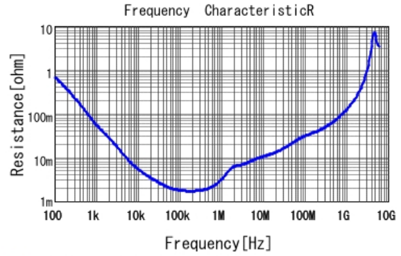
■ GRM21BB30J476ME15 R DCOV, 20degC
